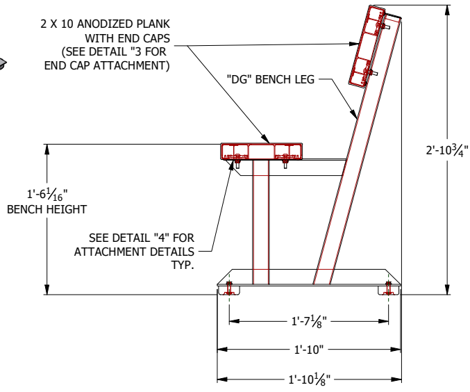
RUBBER FOOT PAD OPTION SEE DETAIL "1"
